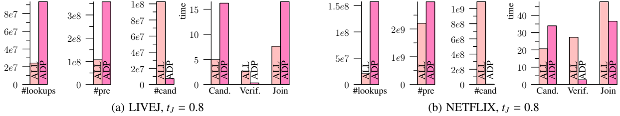
Figure 13: ADP vs. ALL: Candidate generation, verification, and join time.
