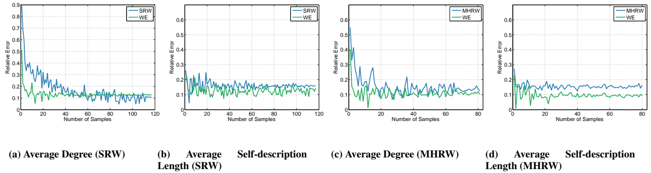
Figure 9: Relative Error of the Average Estimations vs Number of Samples in Google Plus.
