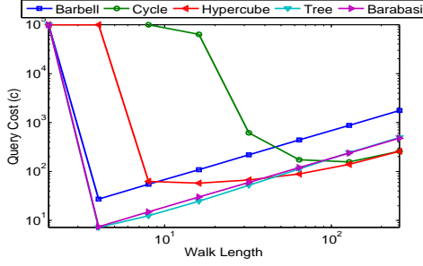
Figure 2: Query cost per sample achieved by IDEAL-AR-SAMPLER.
