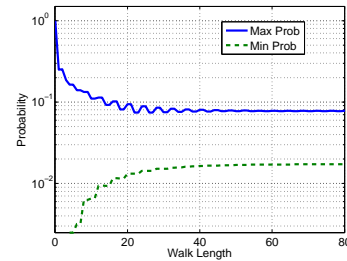
Figure 1: Minimum and maximum probabilities vs walk length
