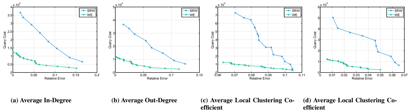
Figure 7: Relative Error of the Average Estimations vs Query Cost in Twitter (from SNAP repository).
