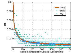
Figure 10: Sampling Distribution in Synthetic Graph
