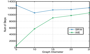
Figure 4: Cycle graphs with long diameter
