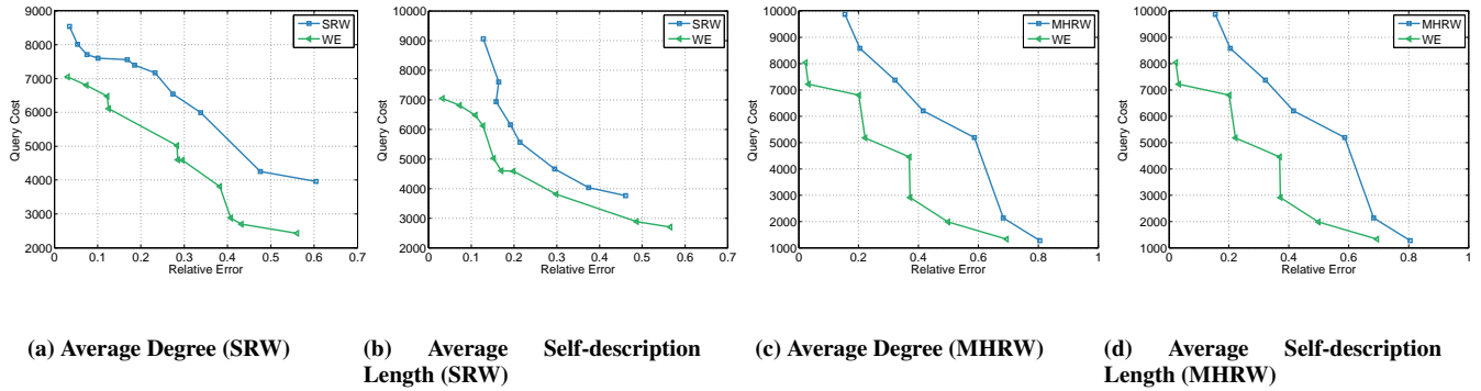
Figure 5: Relative Error of the Average Estimations vs Query Cost in Google Plus.
