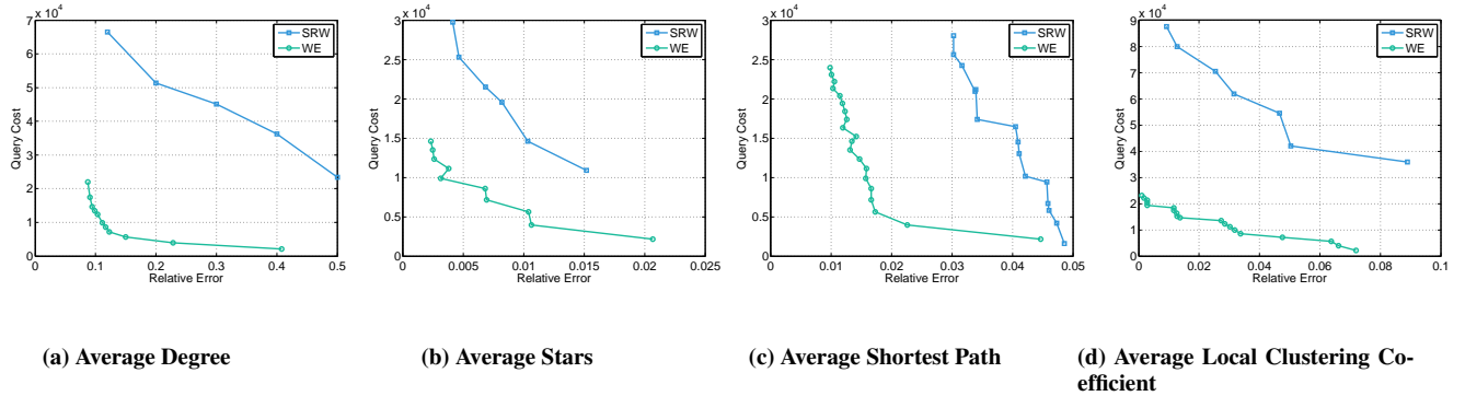
Figure 6: Relative Error of the Average Estimations vs Query Cost in Yelp.
