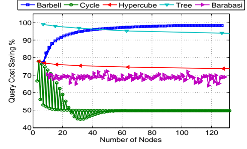
Figure 3: Query cost saving of the IDEAL-AR-SAMPLER.
