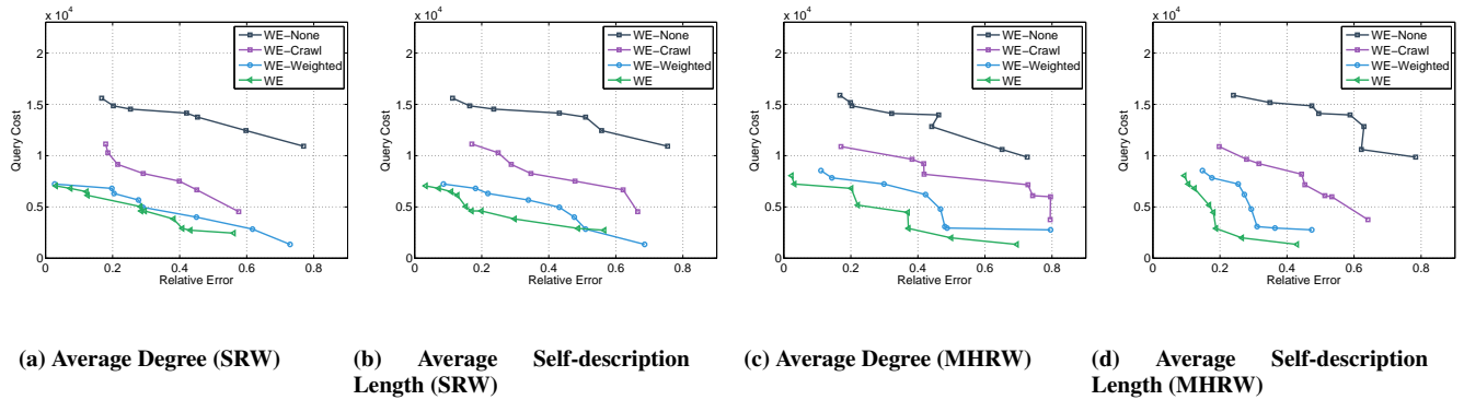
Figure 8: Improvement Trend: Relative Error of the Average Estimations vs Query Cost in Google Plus.
