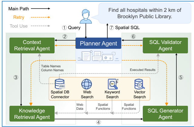
Figure 3: Multi-agent orchestration of SpatialSQL
