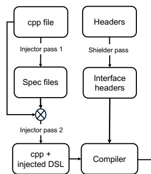
Figure 5: Build-time pipeline.
