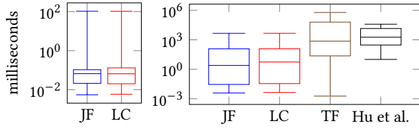
Figure 9: Left: boxplots of runtimes in msec for the query with clause t_1 \leq t_2 . Right: comparison with Hu et al. [28] for point-in-time queries on WikiT.
