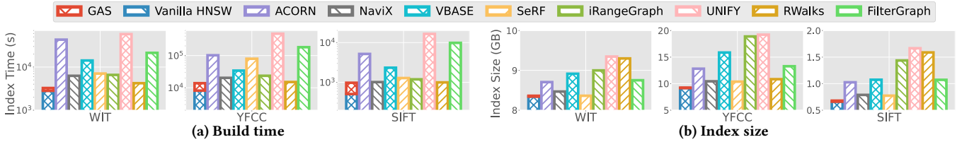
Figure 6: Index construction time and index size of all methods in the single-attribute setting across datasets.
