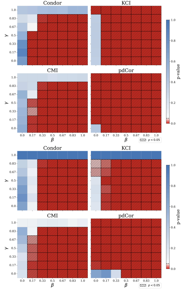
Figure 2: Heatmap of p-values on synthetic data ( n=1000 , k_x=k_t=5 ). Top four heatmaps: d_o=5 , d_p=2 . Bottom four heatmaps: d_o=10 , d_p=5 . Each panel corresponds to one scoring rule; axes report the influence of X on Z ( \gamma ) and of Z on the ranking ( \beta ), and the red/white/blue scale marks respectively strong evidence against, the \alpha = 0.05 boundary, and little evidence against H_0 : R \perp\!\!\!\perp Z | X .
