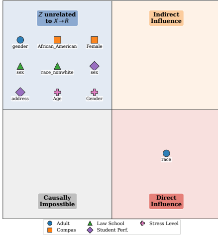
Figure 5: Causal interpretation of CONDOR’s audit on fully black-box models.
