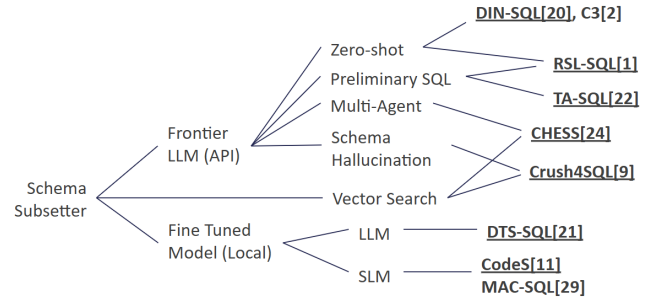
Figure 1: Schema subsetting methods use a variety of techniques and resources including frontier (API-based) LLMs, smaller locally-hosted and finetuned models (both LLM and SLM), and vector search. Some methods use more than one method such as CHESS which uses multiple LLM agents and vector search. Underlined methods indicate that a method is included in our experiments.
