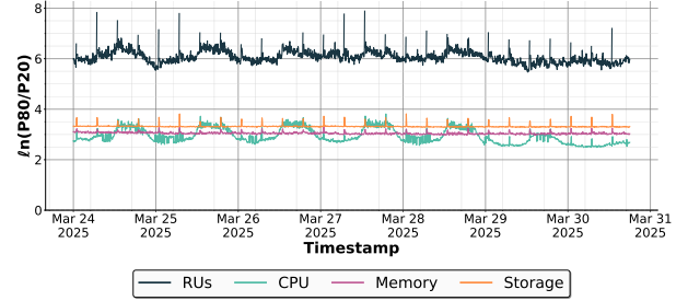
Figure 4: P80/P20 plots for all metrics for Cluster C1b.
