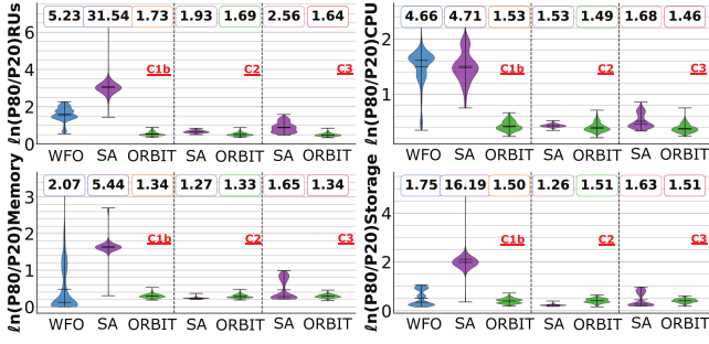
Figure 9: Comparison of \ln\left(\frac{P80}{P20}\right) ratios between ORBIT, WFO and SA. Mean of load (non- \ln ) is shown in label.
