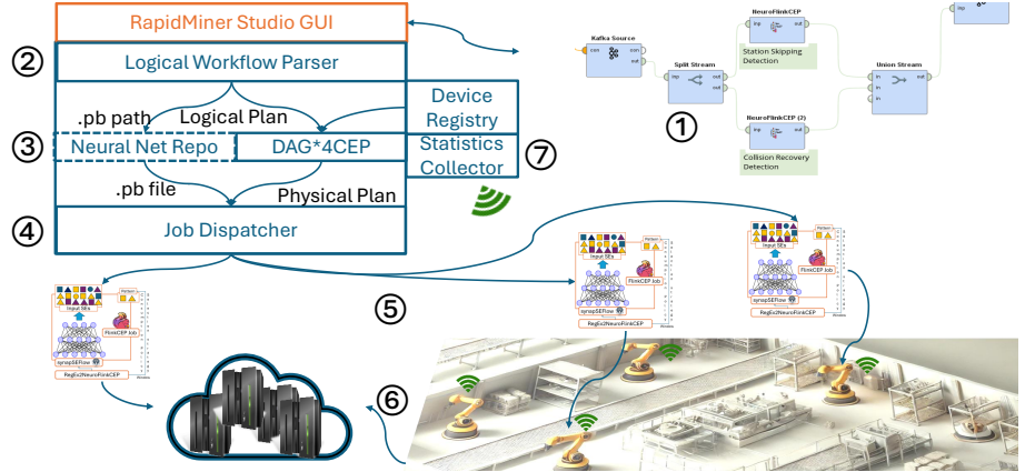
Figure 2: NeuroFlinkCEP Workflow Design, IoT Optimization & Distributed Execution.
