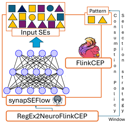
Figure 1: Anatomy of a NeuroFlinkCEP Operator.
