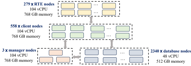
Figure 7: System configuration in TPC-C benchmark
