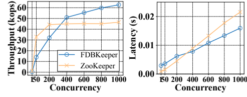
(a) Throughput (b) Latency Figure 9: Performance when reads-to-writes is 9:1.
