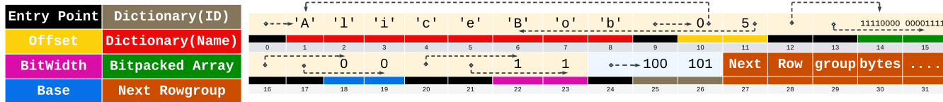
A table with columns Name, Institute, and ID, and gray-inexistent columns including rowgroup, vector, and rowId, indicating which row belongs to which rowgroup and vector. We assign a color to each column, which is also applied to the raw bytes in the FastLanes binary data, depicted at the bottom. The FastLanes file format footer with required fields: Col Name, Type, Offset (representing the binary offset of this column in the row group), Size (allowing computation of the end of the column chunk), Expression (specifying the encoding expression of this column), Metadata, and Segments—an array of two byte ranges [offset, size]. The first range specifies where the segment 'entry point' array (with one entry point per vector) starts within this column chunk and its size, while the second range specifies where the segment data starts and its size.
