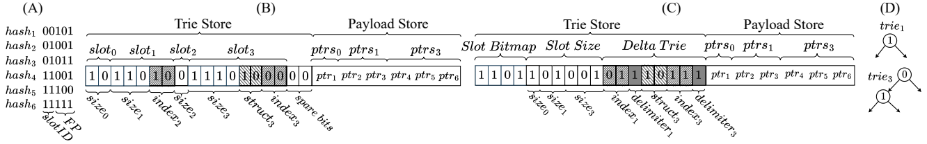
Figure 3: (A) shows the hashes of six keys, where the first two bits encode the slot ID and the rest form the fingerprint. (B) depicts the DHT block design with 4 slots, encoding these keys in the Trie Store and storing sorted payloads in the Payload Store. (C) presents the Sphinx block design with 4 slots, storing the same keys in the Trie Store and sorted payloads in the Payload Store. It consists of a 4-bit Slot Bitmap Segment , indicating whether the trie is empty, followed by a Slot Size Segment for slot sizes and a Delta Trie Segment encoding the topology of each trie. (D) shows the corresponding tries for slot 1 and slot 3 .
