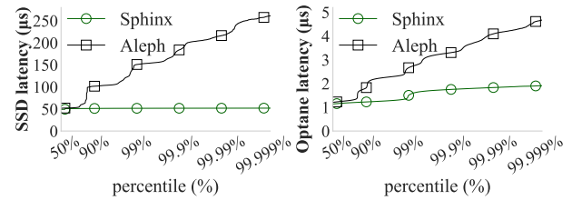
Figure 11: Sphinx maintains stable tail latency even in extreme percentiles.
