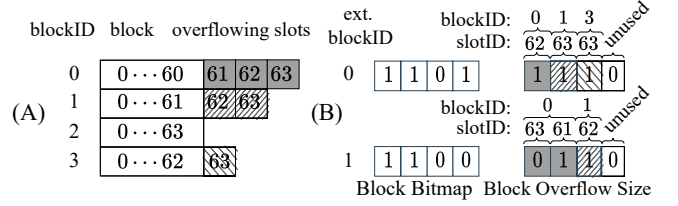
Figure 5: (A) shows 4 blocks, where blocks 0, 1, and 3 have three, two, and one overflowing slots. (B) depicts how the two extension blocks organize their Metadata for these six slots.
