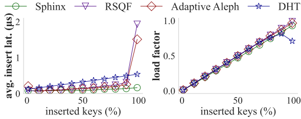
Figure 13: Sphinx exceeds 95% load factor while keeping the most stable and lowest insertion latency.
