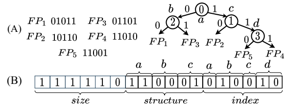
Figure 2: (A) depicts five keys sorted by the first differentiating bit of their fingerprints ( FP_i ), with the fingerprints on the left and the corresponding delta trie on the right. (B) illustrates the physical encoding of the delta trie.
