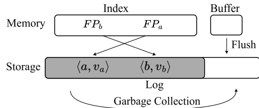
Figure 1: LSH-table streamlines data to storage and stores the location of data entries within an in-memory index.
