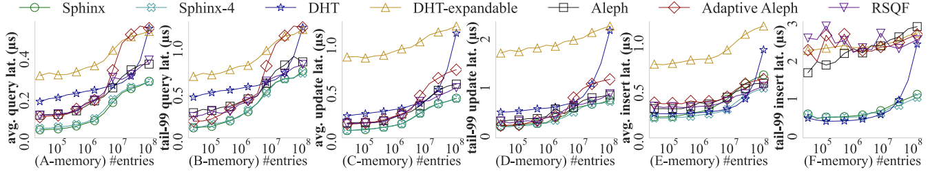
Figure 8: In memory, Sphinx achieves competitive insertion performance and the fastest queries/updates.
