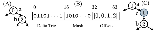
Figure 4: The trie with three entries in Part (A) has the corresponding Decoder entry in Part (B). Part (C) depicts the same trie as in Part (A) with a non-differentiating node c .
