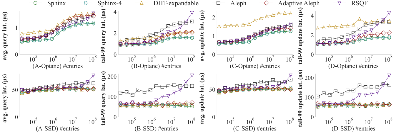
Figure 9: On Optane, Sphinx variants are fastest; on SSD, they match or beat all baselines by avoiding false positives.
