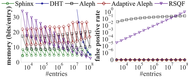
Figure 6: Sphinx eliminates false positives, uses at most half the memory of other baselines, and maintains a stable memory footprint while scaling.
