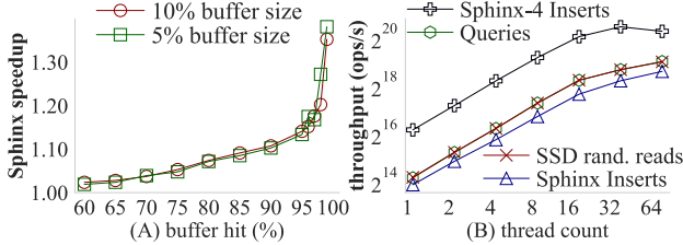
Figure 10: (A) Sphinx leads to substantial benefits with SSD under workload skew. (B) Sphinx scales well with threads.
