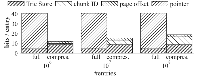
Figure 7: Compressing pointers reduces the pointer overhead and signifies the total memory efficiency of Sphinx.
