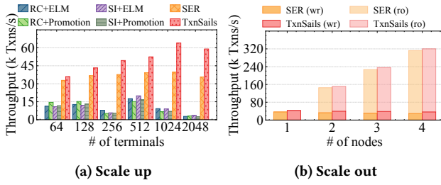
Figure 17: Scalability in Neon - YCSB
