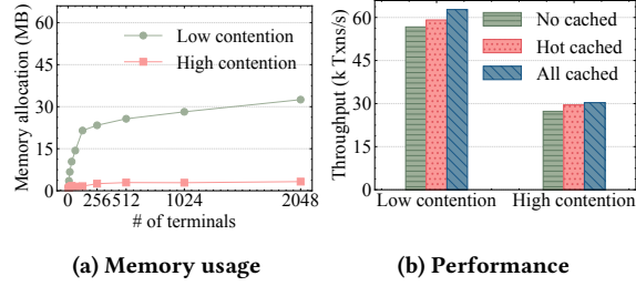
Figure 10: Impact of Metadata - YCSB
