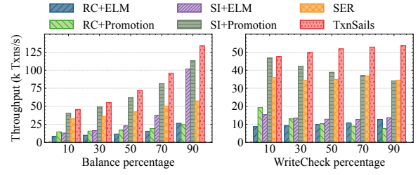
Figure 14: Impact of templates percentage - SmallBank
