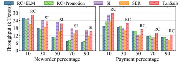
Figure 15: Impact of templates percentage - TPC-C
