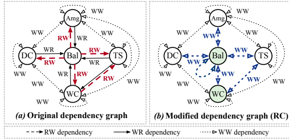
Figure 1: Static dependency graphs of Smallbank
