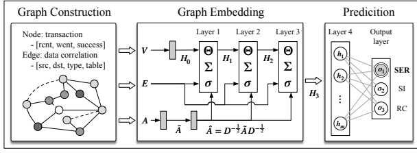
Figure 4: Graph-based isolation level selection model
