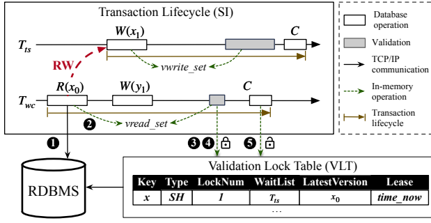
Figure 3: Transaction processing in TxNSAILS
