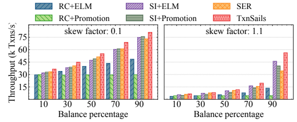
Figure 16: Extended evaluations on MySQL - SmallBank
