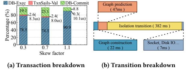
Figure 7: Breakdown analysis - YCSB
