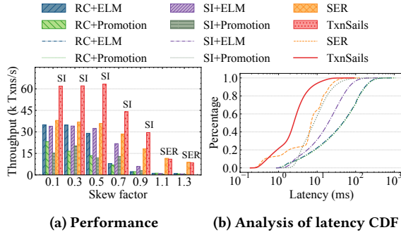
Figure 12: Impact of data contention - YCSB
