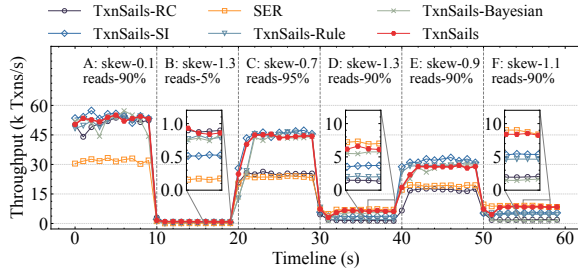
Figure 6: Workload shifting - YCSB
