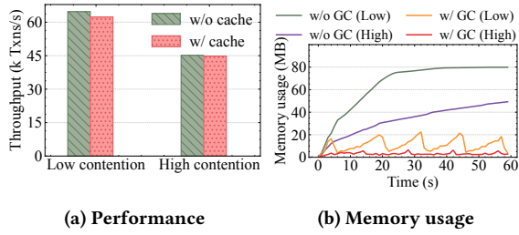
Figure 9: Impact of garbage collection - YCSB
