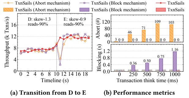
Figure 8: Comparison of transition mechanisms - YCSB
