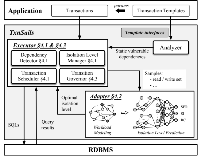
Figure 2: An overview of TxnSAILS
