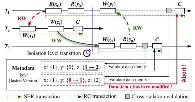
Figure 5: Cross-isolation validation
