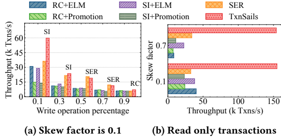
Figure 13: Impact of write/read ratio - YCSB
