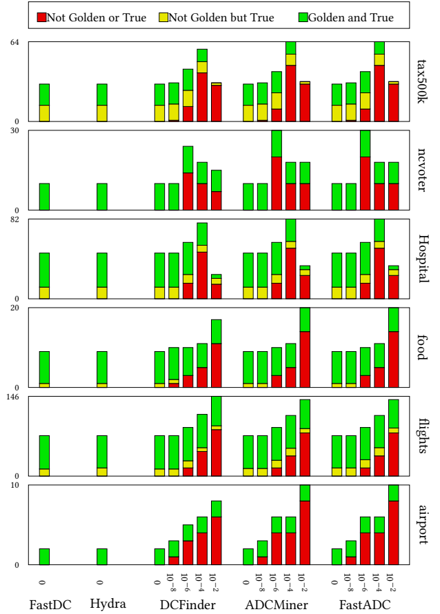
Figure 7: Number of discovered sound DCs that are golden and those that are true despite not being golden. Shows how sound DCs almost entirely correspond to true data constraints, unlike those shown in Figure 2.
