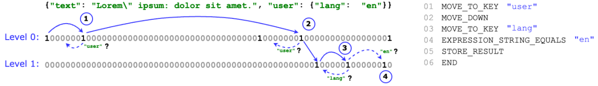
Figure 3: Index traversals during query execution and generated bytecode for the query $.user[?(@.lang == "en")]
