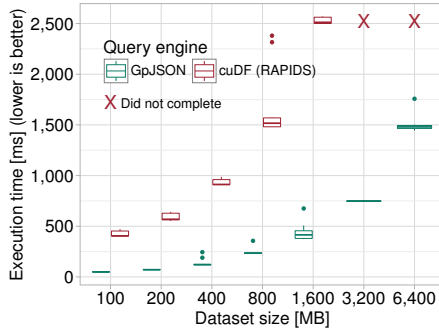
Figure 8: Comparing GpJSON to the cuDF library on the A6000. The cuDF library errored for the two largest files.
