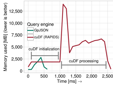
Figure 9: Memory usage of GpJSON vs. cuDF. cuDF execution is further split into two stages.
