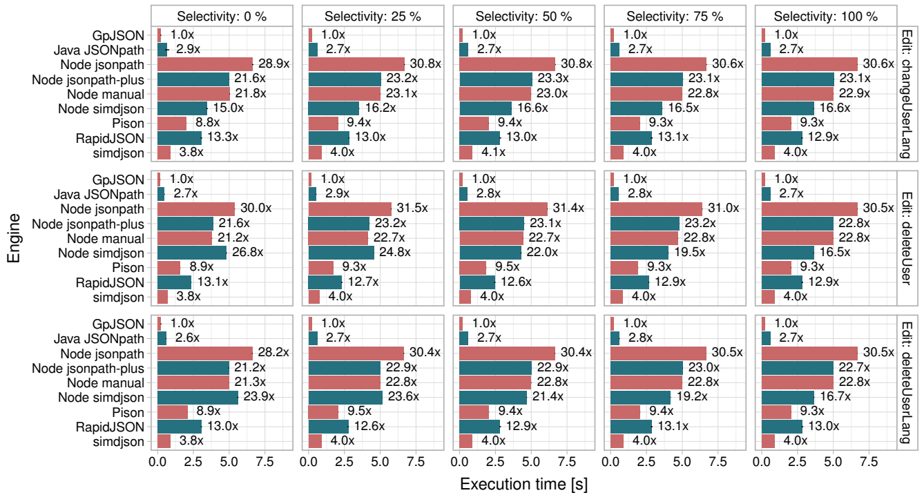
Figure 6: Comparison between GpJSON running on A100 (GPU4.8) and libraries running on the HPC shape. The dataset has been edited in different ways to change the number of matches during query execution. Lower is better.
