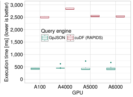
Figure 10: Performance of GpJSON and cuDF across different GPUs. File size was fixed at 1,600MB.
