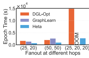
Figure 16: Performance under different sampling fanouts and hops.
