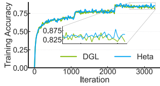
(b) MAG240M dataset
