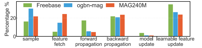
Figure 4: Percentage of the epoch time spent on each stage: training R-GCN on three datasets with DGL.
