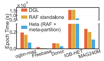
Figure 14: Meta-partitioning different GPU numbers. Heta significantly enhances RAF’s effectiveness.
