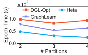
Figure 13: Performance under different GPU numbers. Heta significantly enhances RAF’s effectiveness.
