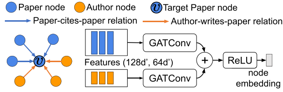
Figure 1: Illustration of relation-specific aggregation in R-GAT [3]. In an academic network, a target paper node aggregates features separately along two different relations.
