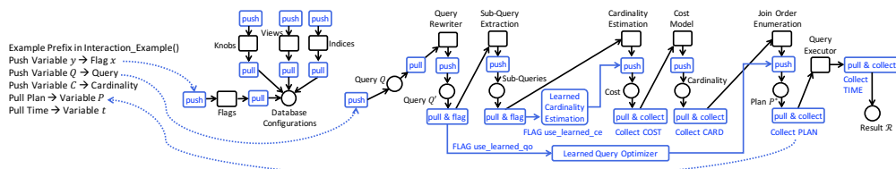
Figure 10: Workflow of query processing with anchors added by PilotScope.
