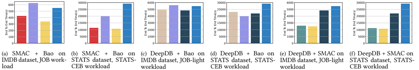
Figure 12: End-to-end execution time of multiple AI4DB algorithms on PostgreSQL.
