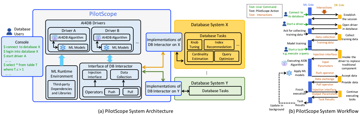
Figure 2: System architecture and workflow of PilotScope.
