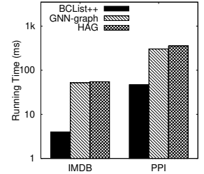
Figure 11: Evaluating GNN information aggregation
