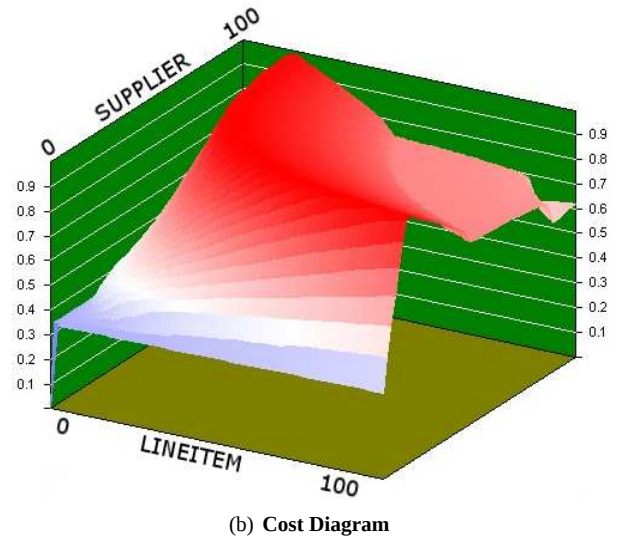
Figure 12: Intra-plan Non-Monotonic Costs (Query 21, OptA)
