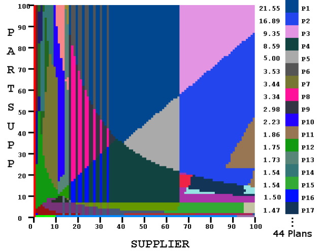
Figure 8: Venetian Blinds Pattern (Query 9, OptB)
