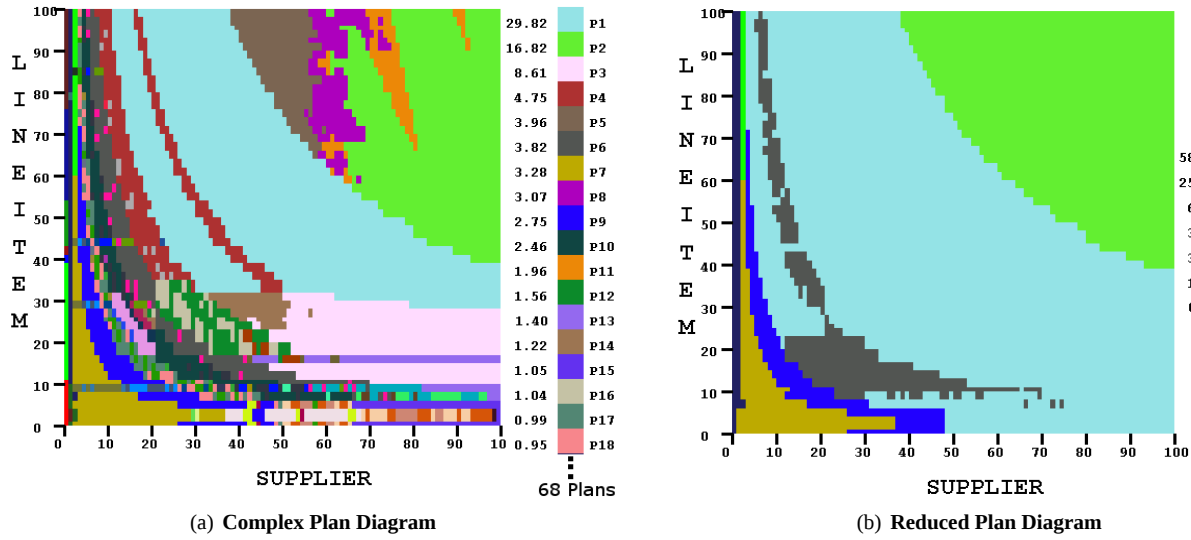
Figure 2: Complex Plan and Reduced Plan Diagram (Query 8, OptA)
