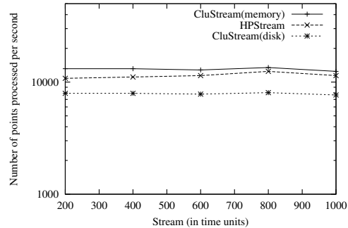
Figure 11: Stream Processing Rate (Network Intrusion data set, stream_speed = 200)
