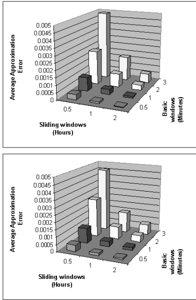
Figure 4: Average approximation errors for correlation coefficients with different basic/sliding window sizes for synthetic(above) and real(below) datasets
