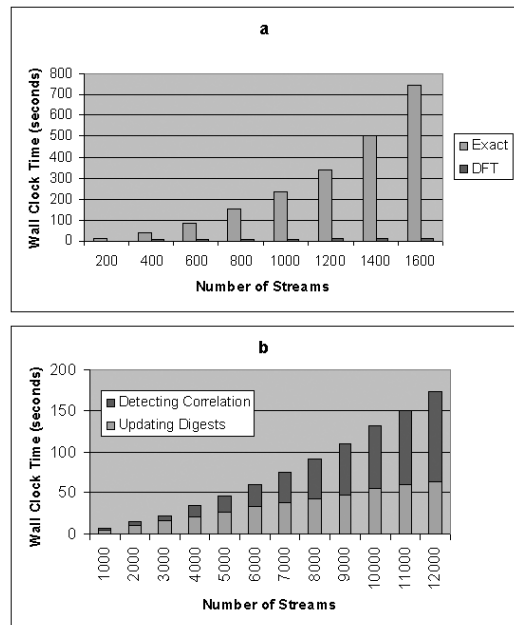
Figure 2: Comparison of the number of streams that the DFT and Exact method can handle
