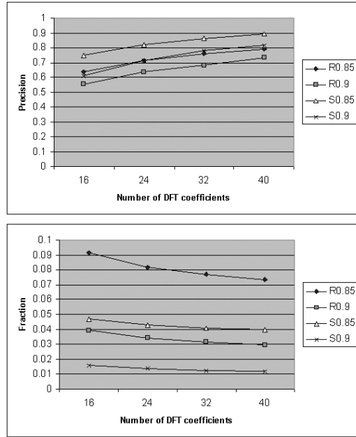
Figure 5: The precision and pruning power using different numbers of coefficients, thresholds and datasets
