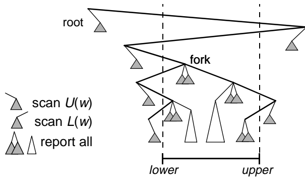
Figure 7: Query processing in the interval tree.
