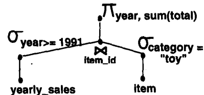
Figure 11: Optimizing after replacing Q with Q'
