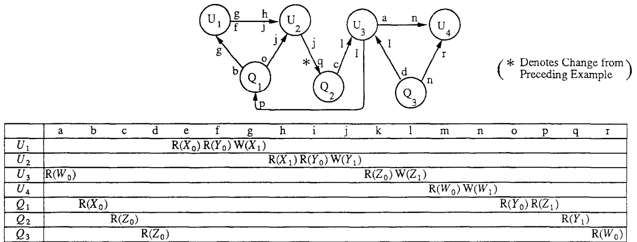
Figure 2.3: A Schedule and Serialization Graph Illustrating Weak Consistency for Queries
