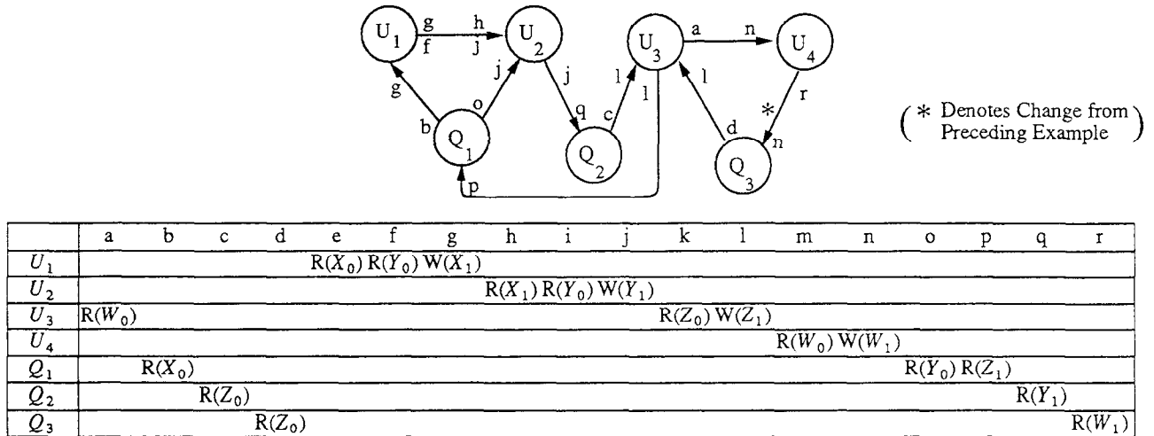
Figure 2.4: A Schedule and Serialization Graph Illustrating Update Consistency for Queries
