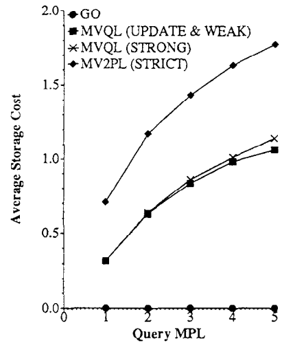
Figure 5.9: Average Storage Cost
