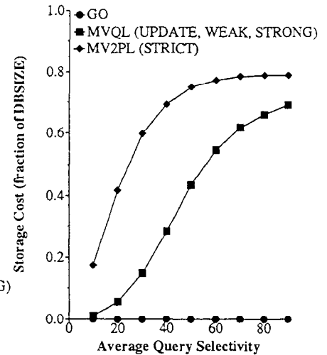
Figure 5.3: Average Storage Cost
