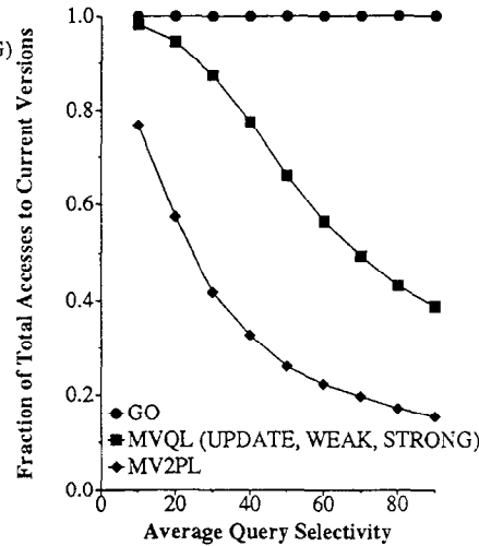
Figure 5.2: Current Version Access
