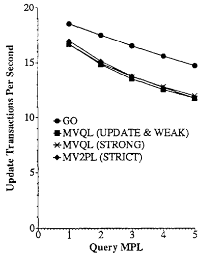
Figure 5.8: Update Transaction Throughput
