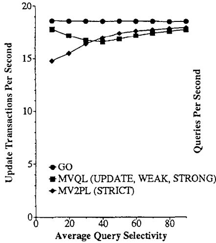
Figure 5.4: Update Transaction Throughput (Update Transaction Size = 2) ( MPL_{query} = 1, MPL_{update} = 12 )
