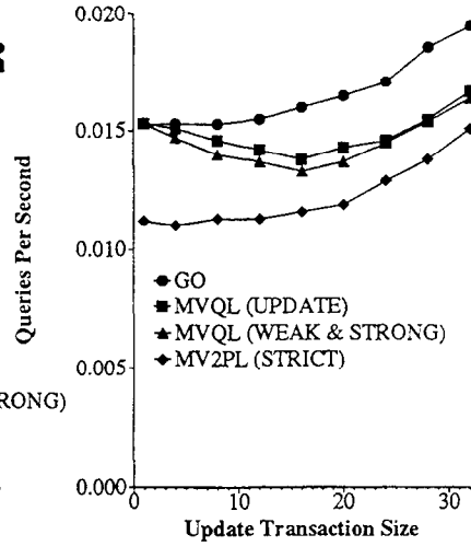
Figure 5.5: Query Throughput ( Selectivity_{Query} = 25\% ) ( MPL_{query} = 1, MPL_{update} = 12 )
