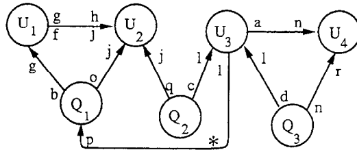
Figure 2.1: A Schedule and Serialization Graph Illustrating Strict Consistency for Queries
