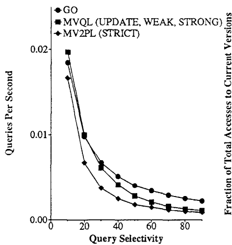
Figure 5.1: Query Throughput
