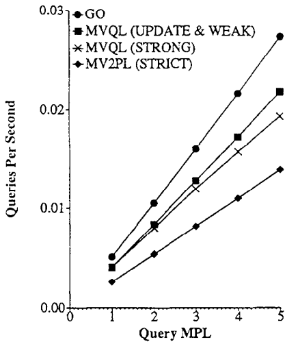
Figure 5.7: Query Throughput
