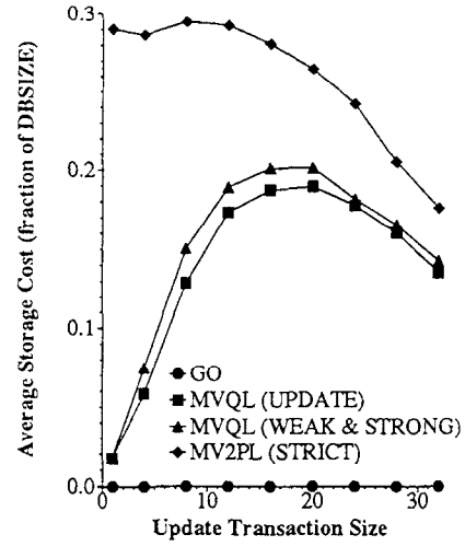
Figure 5.6: Average Storage Cost ( Selectivity_{Query} = 25\% ) ( MPL_{query} = 1, MPL_{update} = 12 )
