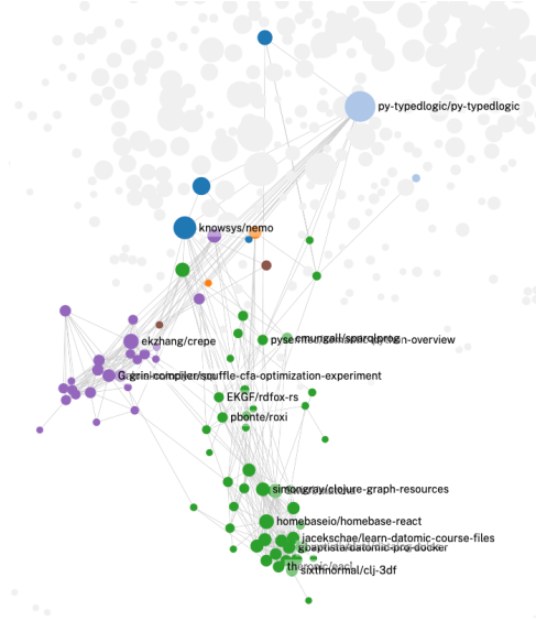
Figure 2: The colored nodes represent 98 repositories tagged with the "Datalog" topic, connected by 388 edges. Gray nodes (not all are shown) represent the remaining repositories in the corpus \mathcal{R}' for logic programming. An edge is drawn between two repositories if they share at least one logic programming topic (e.g., Prolog). Node size reflects an importance score computed using PageRank. Of particular interest is the repository "py-typedlogic", which, despite representing a relatively small community, shares several topics with other repositories.
