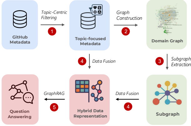
Figure 1: DeepGit follows a five-step process: (1) building a topic-focused knowledge base from GitHub metadata, (2) constructing a domain graph, (3) extracting subgraphs, (4) fusing data into a hybrid representation, and (5) enabling question answering via GraphRAG.
