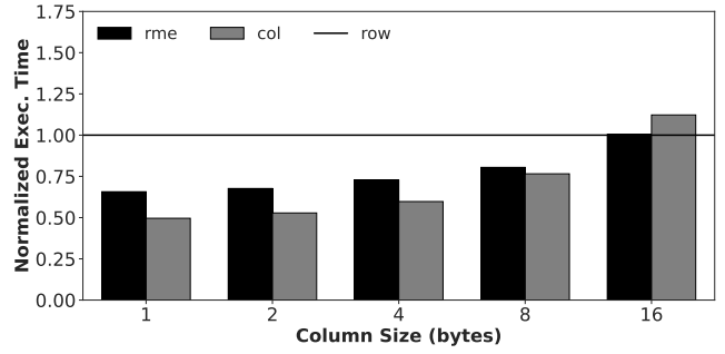
(a) Executing Q0: RME outperforms row-store for column sizes up to 8 bytes. We also observe that prefetching is more beneficial for RME vs. column-store for low column sizes.
