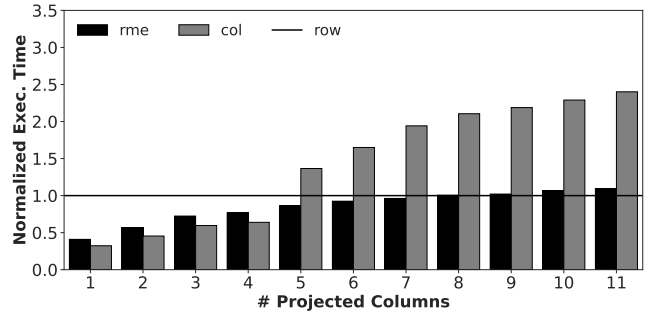
(b) Executing Q1: Turning off hardware prefetching affects RME, however, it does not change the high-level trends. For increased projectivity, the tuple reconstruction cost kicks in, making RME substantially faster than column-store. Further, the lack of prefetching makes row-store for high projectivity more competitive than RME.
