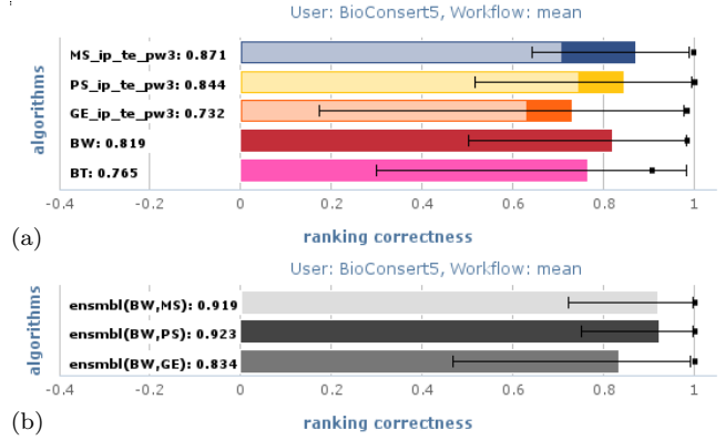
Figure 9: Mean ranking correctness for (a) single algorithms’ best configurations (shaded: baseline evaluation, see Fig. 5), and (b) the best ensembles of two (see text).
