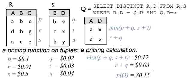
Figure 1: Query price derivation for a tuple-based pricing scheme using the pricing semiring formalism.
