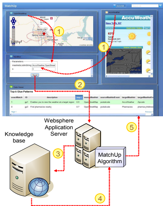
Figure 2: Architecture and flow
