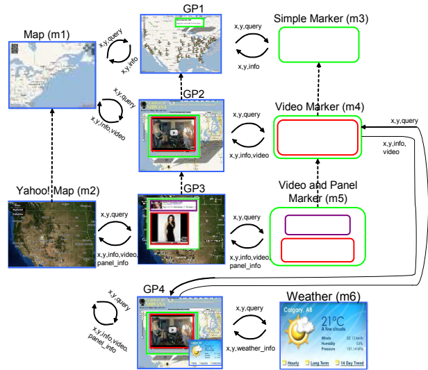
Figure 1: Inheritance of Mashlets and Glue Patterns
