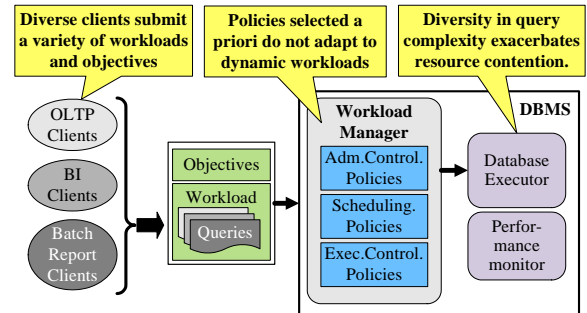
Figure 1: Architecture of management today: Traditional workload management can compensate for short-term problems, but cannot adapt policies in the presence of longer-term problems caused by (dynamic) changes in the workload.
