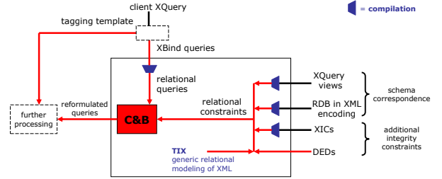
Figure 3: MARS architecture
