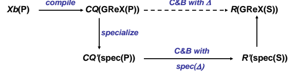
Figure 7: Reformulation by schema specialization
