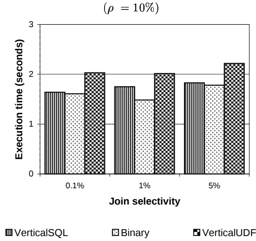
Figure 10: Join performance (1000 cols × 20K rows)
