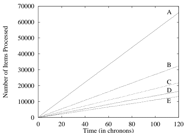
Figure 7: Performance of sequential scan, Rate metric
