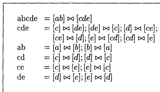
Figure 7: MEMO-structure in which [ab] \bowtie [cde] is about to be explored.
