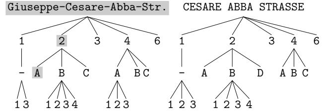
Figure 3: Address trees of streets 30 from R0 and 91 from LR.
