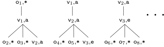
Figure 6: Some of the 2,3-grams of \mathbf{T}_1 .
