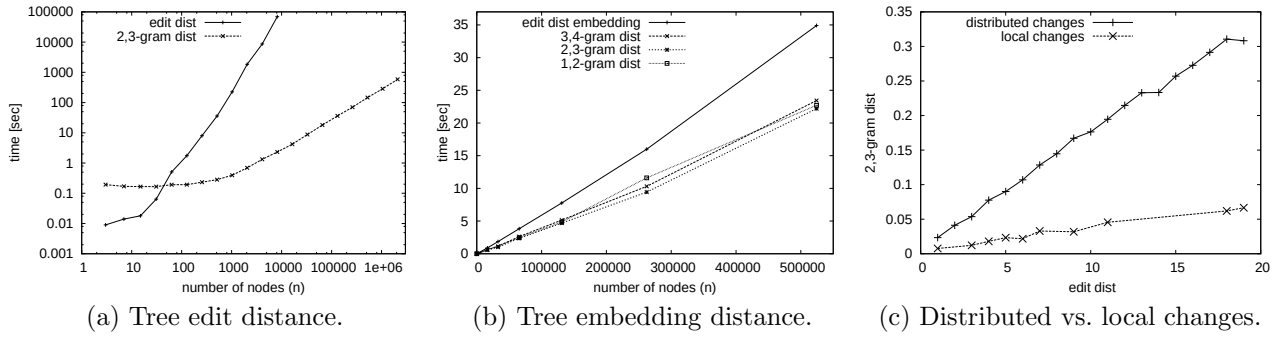
Figure 14: Scalability results and subtree deletions.
